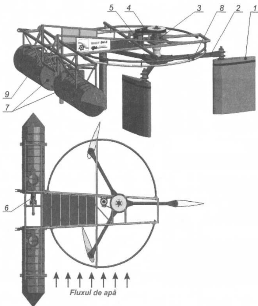
Figure 4: Micro-hydro power plant with hydrodynamic rotor river water kinetic energy conversion into electrical and mechanical energy (rotor diameter D = 4\text{m} , water-submersed blade height h = 1,4\text{ m} , length of the blade cord l = 1,3 ).
